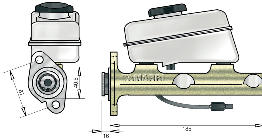
PF369 / Olio freni DOT3-4 - Brake oil DOT3-4 Con 2 uscite olio (sx) / With 2 exit oil(lh) Hyster
