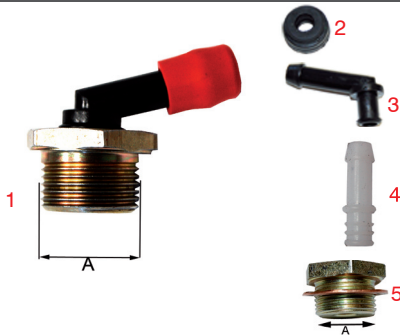
Raccordo pipa per pompe Plug connection for pumps
